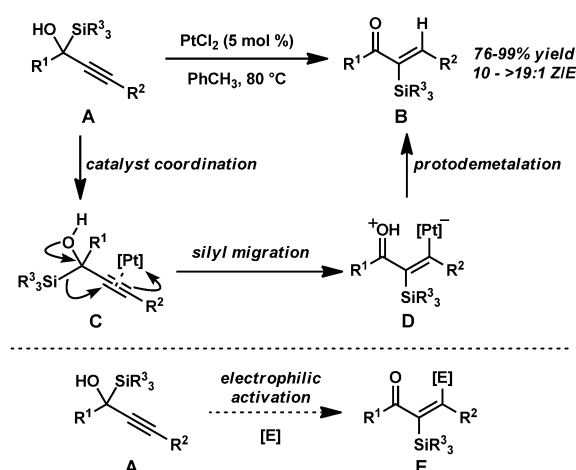
Figure 1. Pt-catalyzed anti -selective silicon migration to form ( Z )- \alpha -silylenones.
