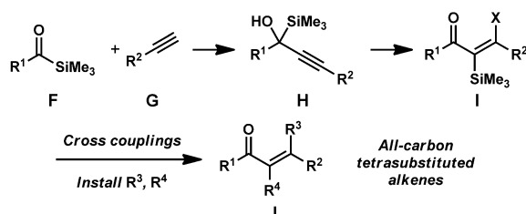
Figure 2. Modularity of the all-carbon tetrasubstituted alkene synthesis.
