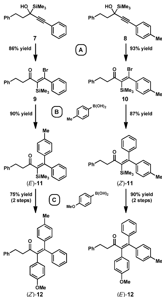
Scheme 2. Selective formation of ( Z )- and ( E )-isomers of alkene 12 . Step A: NBS (1.1 equiv), \text{CH}_2\text{Cl}_2 , -78 \rightarrow 0^\circ\text{C} (for 7 ) or 0^\circ\text{C} (for 8 ). E/Z ratios: 9 : > 19:1; 10 : > 19:1. Step B: \text{ArB}(\text{OH})_2 (2.0 equiv), (\text{Ph}_3\text{P})_2\text{PdCl}_2 (0.05 equiv), \text{Cs}_2\text{CO}_3 (10 equiv), 1,4-dioxane/ \text{H}_2\text{O} , 50^\circ\text{C} . Step C: 1) \text{ICl} (1.1 equiv), \text{CH}_2\text{Cl}_2 , -78^\circ\text{C} ; 2) \text{ArB}(\text{OH})_2 (2.0 equiv), (\text{Ph}_3\text{P})_2\text{PdCl}_2 (0.05 equiv), \text{Cs}_2\text{CO}_3 (10 equiv), 1,4-dioxane/ \text{H}_2\text{O} , 50^\circ\text{C} . E/Z ratios: ( Z )- 12 : 1:10.4; ( E )- 12 : 11.3:1.
