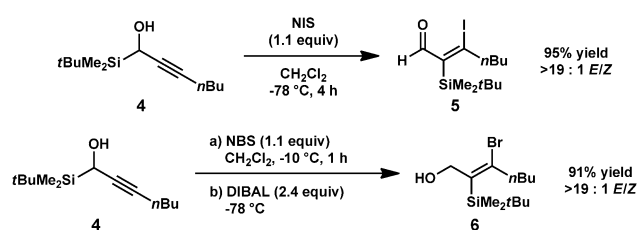
Scheme 1. Reactivity of secondary \alpha -hydroxypropargylsilanes.
